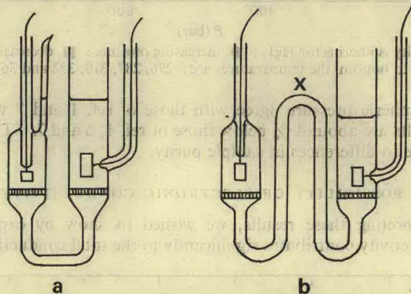
FIG. 7.—Cells used for electrolysis experiments on fused HgI 2 .
